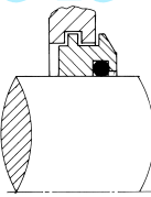
TENUTA A LABIRINTO "TSNS" PER SUPPORTI: SNG-SNU "TSNS" LABYRINTH SEAL FOR: SNG-SNU TYPE
