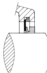
TENUTA V-RING "TSNA" PER SUPPORTI: SNG-SNU "TSNA" V-RING SEAL FOR: SNG-SNU TYPE
