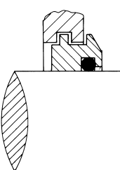
TENUTA A LABIRINTO "TSNS" PER SUPPORTI: SNG-SNU "TSNS" LABYRINTH SEAL FOR: SNG-SNU TYPE
