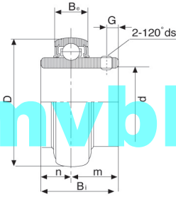
ZUC200 (Normal Duty) Spherical O.D.
