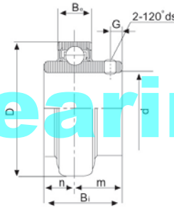
CUCX00L3 (Medium Duty) Cylindrical O.D.
