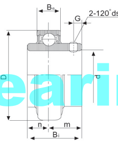
CUC200L3 (Normal Duty) Cylindrical O.D.
